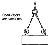
Hook Slings
