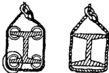
Good - Sharp corners padded.
