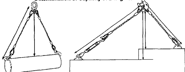
Determination of Capacity of 2-Leg Bridle Hitch
