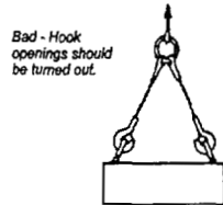
Double slings shall be used when hoisting 2 or more pieces of material over 12 ft long.
